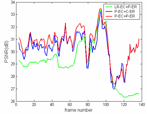
Figure 7. Recovery performance of three combinations. QCIF Foreman sequence, HR bit-rate=91kbps, LR bit-rate=19kbps, 3 consecutive frames per loss.
