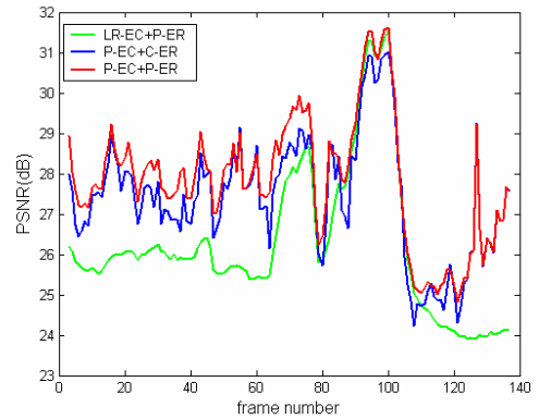
Figure 8. Recovery performance of three combinations. QCIF Foreman sequence, HR bit-rate=91kbps, LR bit-rate=11kbps, 3 consecutive frames per loss.
