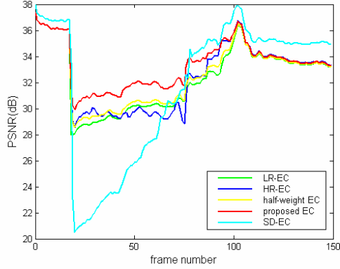
Figure 5. The recovery of PSNR after the lost 18 th , 19 th and 20 th HR frames.
