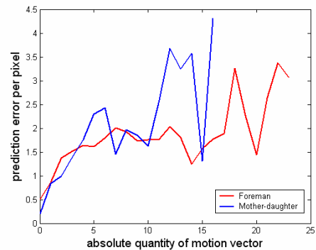
Figure 1. Statistical correlation between motion vector and prediction error. QCIF sequences, 15fps(150frames), JM86.
