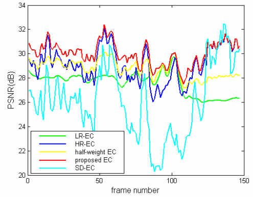
Figure 3. Concealment performance of five methods. QCIF Foreman sequence, HR bit-rate=91kbps, LR bit-rate=19kbps, SD bit-rate=111kbps, 3 consecutive frames per loss.
