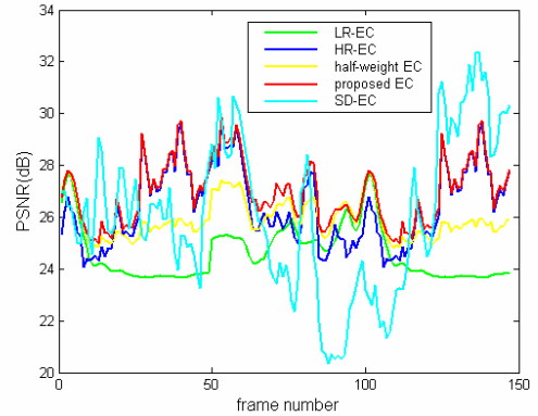
Figure 4. Concealment performance of five methods. QCIF Foreman sequence, HR bit-rate=91kbps, LR bit-rate=11kbps, SD bit-rate=104kbps, 3 consecutive frames per loss.
