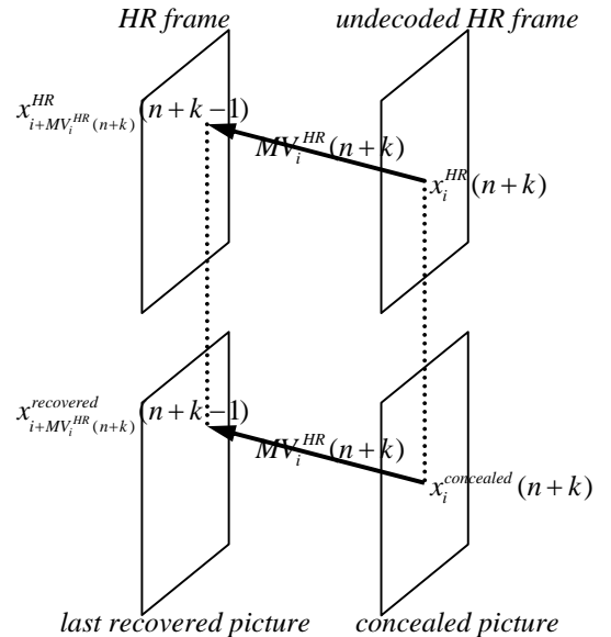
Figure 2. Two pairs of dependent pixels, as a computational unit of the interframe error recovery algorithm.
