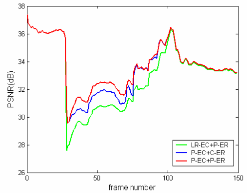
Figure 9. The recovery of PSNR after the lost 28 th , 29 th and 30 th HR frames.
