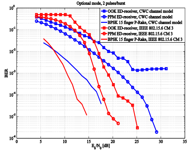
Figure 5. BER with an optional mode, 2 pulses/burst.
