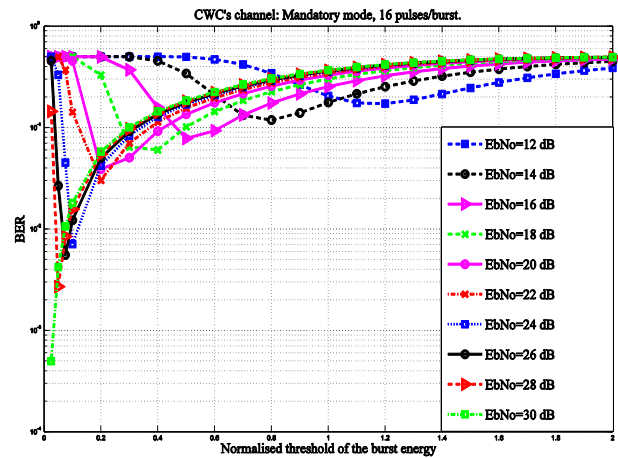
Figure 3. OOK energy thresholds with some E_b/N_0 values.
