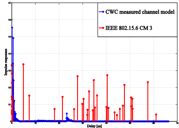
Figure 1. Impulse responses of the used IEEE 802.15.6 CM3 and CWC channel models.
