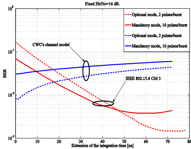
Figure 2. Effect of extension of the integration interval on receiver bit error performance.
