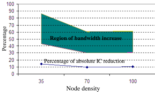
Figure 2: Green region shows capacity increase by using random initialization before the channel self-organization is invoked – (refer 4.1.1). Note: The percentage of IC reduction i.e. blue line and bandwidth are illustrated together to show the significant improvement that results by using random initialization algorithm.
