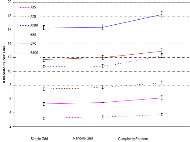
Figure 1: 98% bounds of absolute interference cost per link (A-after self-organization, B-before self organization)
