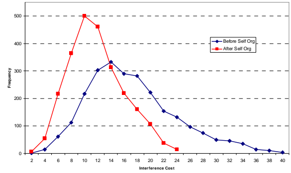
Figure 3: IC across the network before (blue) and after (red) self-organization–random initialization algorithm.
