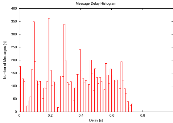
Figure 5: Delay histogram; synchronized network ( \delta = 50ms ).
