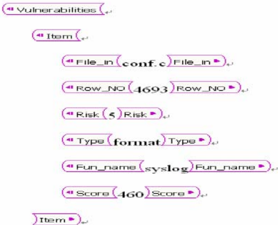
Fig.5 a XML description of one vulnerability entry
