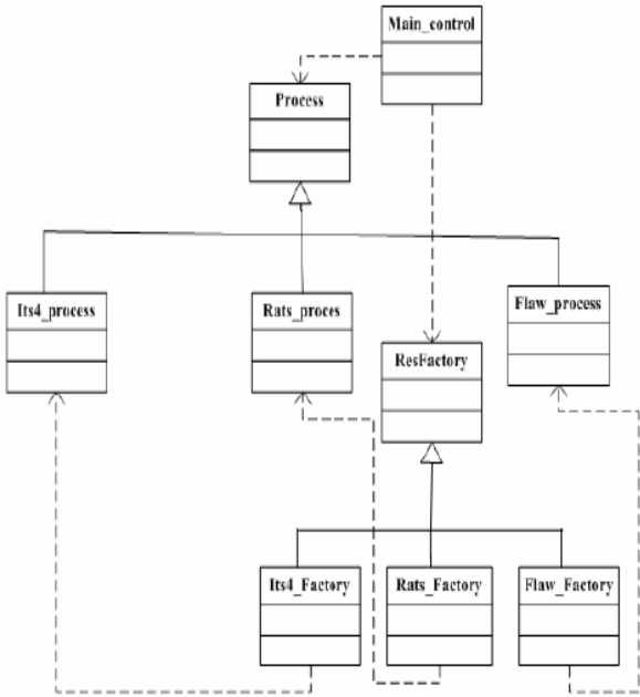
Fig.4.class diagram of ISA (partly)
