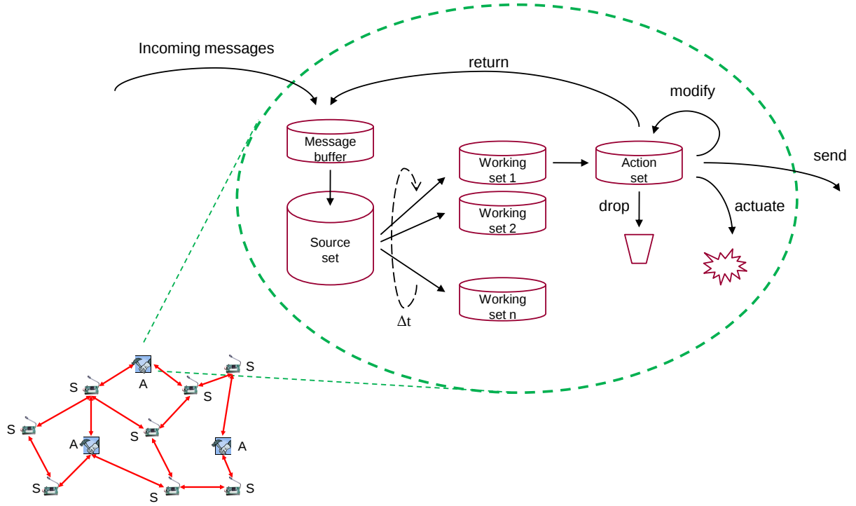
Figure 3: The working behavior of a single RSN node. Received messages are stored in a buffer, selected to a working set according to specific criteria, and finally processed, i.e. forwarded, dropped, etc.
