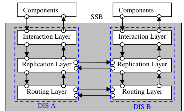
Fig. 3: Architecture of an SSB and interaction with components
