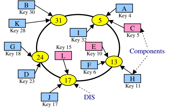
Fig. 2. Chord based SSB in a circular keyspace with m=5 .
