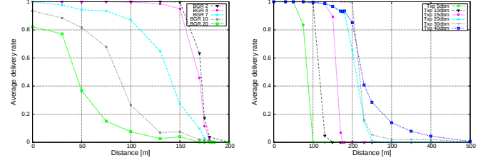
(a) Average BDR vs. distance varying BGR Average (b) Average BDR vs. distance varying transmission power
