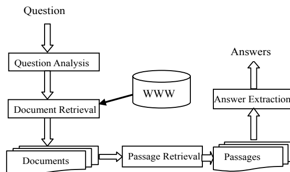
Figure 1. Architecture of our web-based QA system
