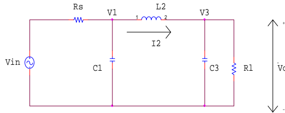
Fig.2: Doubly Terminated LC Ladder Filter (Low pass Section)
