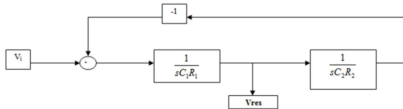
Fig.4: Block Diagram of Resonant Section
