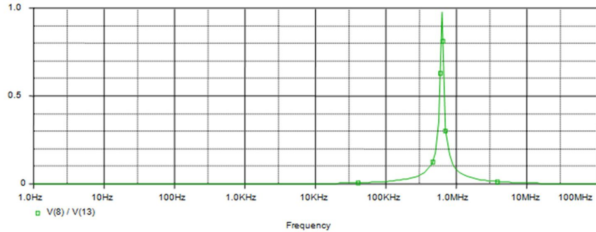
Fig.8: Response of Second Order Resonance Section
