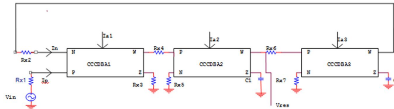
Fig.5: Circuit Realization of Resonant Section Using CCCDBA
