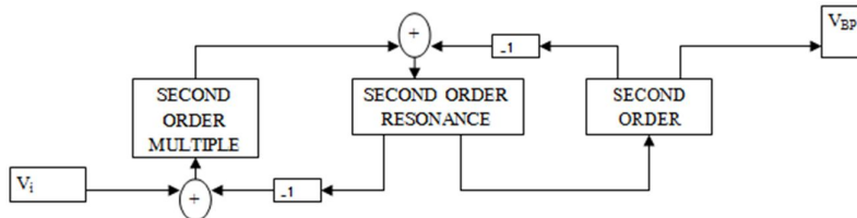
Fig.6: Block Diagram of Sixth Order Leapfrog Filter (Bandpass Section)
