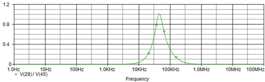
Fig.9: Response of Sixth Order LC Ladder Band Pass Filter
