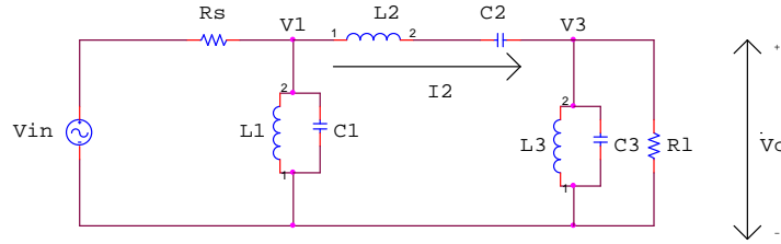
Fig.3: Doubly Terminated LC Ladder Filter (Band pass Section)
