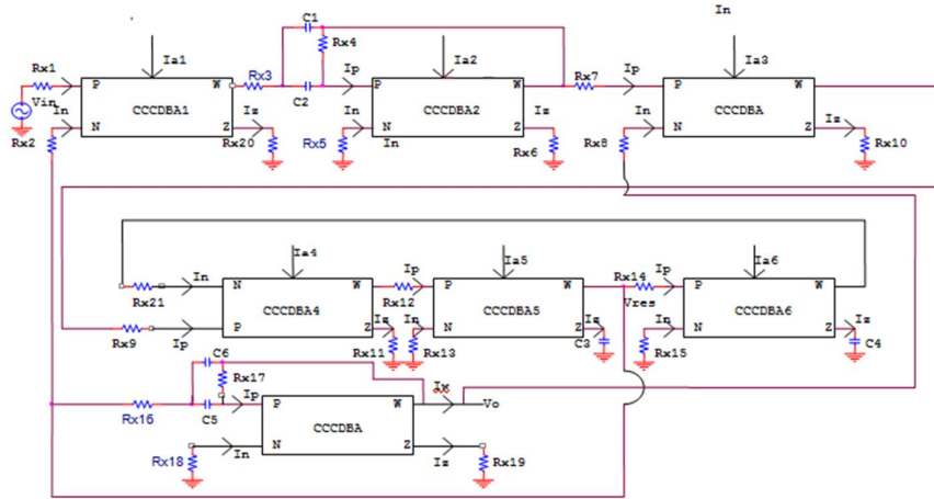
Fig.7: Circuit Diagram of Sixth Order Doubly Terminated LC Ladder Leapfrog Band pass Filter Using CCCDBA
