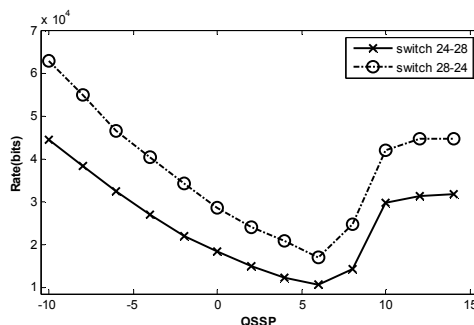
Figure 3. Bit rate of SSP-frames
