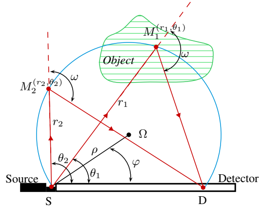
Figure 2: Principle of Norton's CST
