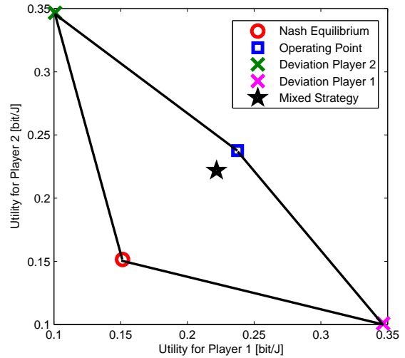
Figure 4: Nash Equilibrium, Operating Point and the Deviation Utilities for (K, M, N) = (2, 2, 2)
