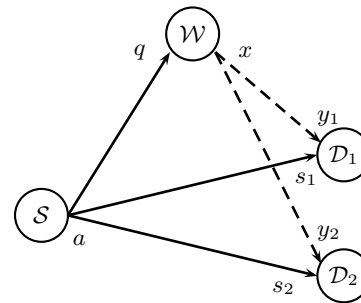
Figure 1: Interpreting the monitoring structure of a dynamic game as a communication problem.
