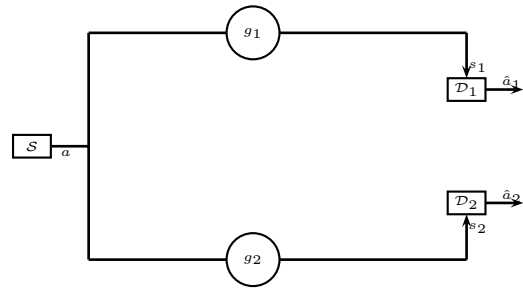
Figure 2: The private monitoring channel.
