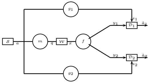
Figure 3: The mediator-assisted monitoring channel.
