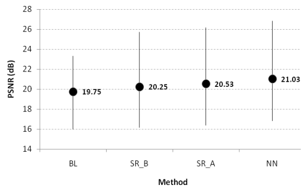
Fig. 7. Average PSNR results, 8\times zoom factor.
