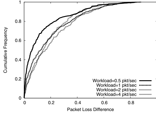
Fig. 4. Packet Loss Difference for Pairs of Nodes (taken from [14])
