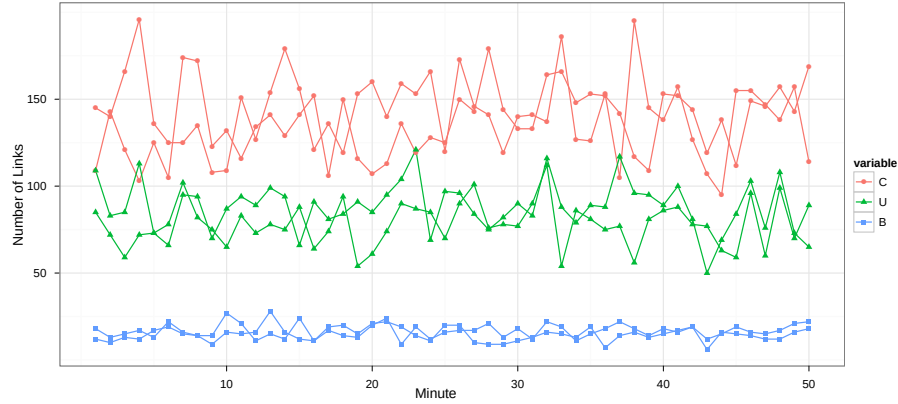
Fig. 14. Measured Links on the lawn for Channels 0 and 3: (C)changes, (U)unidirectional ones, (B)idirectional ones
