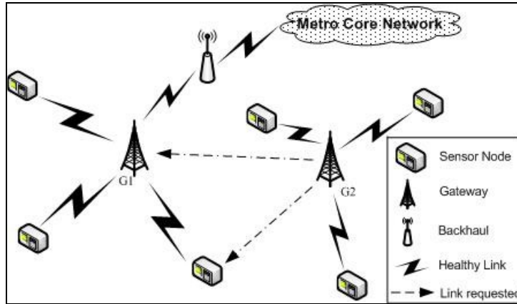
Fig. 8. Illustration of the scenario of a gateway attempting to reestablish connection to the backhaul through a bridging gateway or a sensor node.
