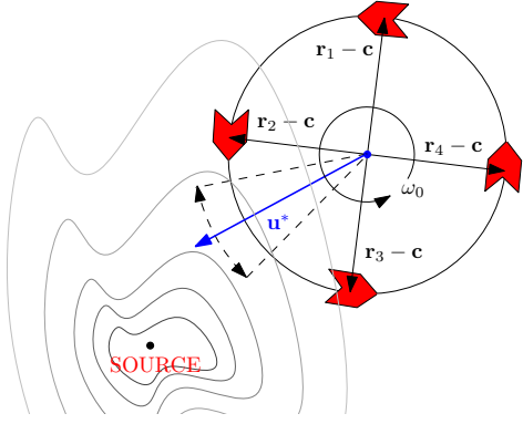
Figure 1: Problem formulation
