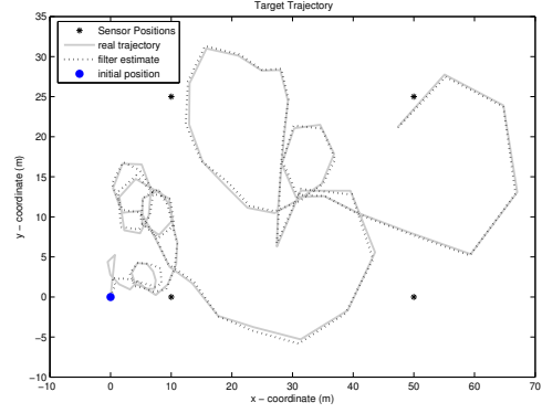
Fig. 8. True and filtered trajectory - ROT-MMPF Scenario 2
