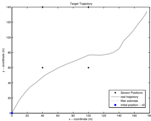
Fig. 2. True and Filtered target trajectory - ROT-PF Scenario 1
