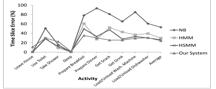
Fig. 4: Comparison of Time Slice Error for Activity Recognition among different classifiers.
