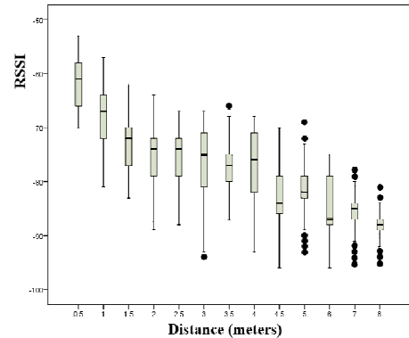
Figure 1. RSSI dependence on the distance
