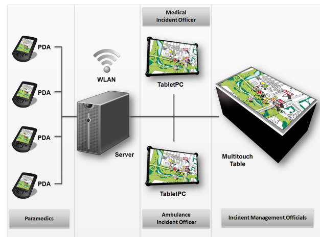
Fig. 1. UI concept: Paramedics are equipped with PDAs in order to track the patients indirectly. Paramedics, ambulance incident officer and medical incident officer are tracked directly via their devices (PDA, tablet PC). All positions are shown on the multitouch table in order to manage the MCI.
