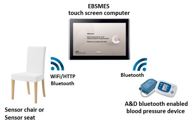
Figure 1. When a test-subject is seated the system monitors activity and posture and starts recording audio data. When a BP measurement is received the audio data is processed and classified as speech or silence.
