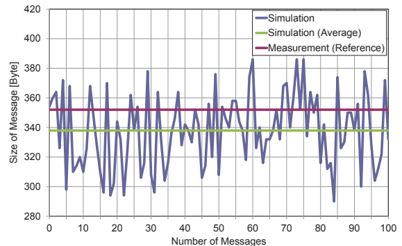
Figure 5: Analysis of Metering Data Format (SML-geListResponse)
