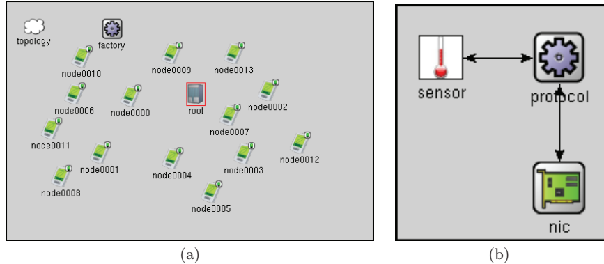
Figure 1: (a) An example simulation scenario. (b) The components of a modelled node in the scenario.
