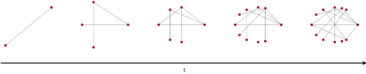
Figure 3: g_{n,p} graph growth. p = 0.2 .
