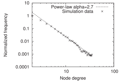
Figure 5: \log\text{-}\log plot of average node degree over all the data series shown in Figure 4(b).
