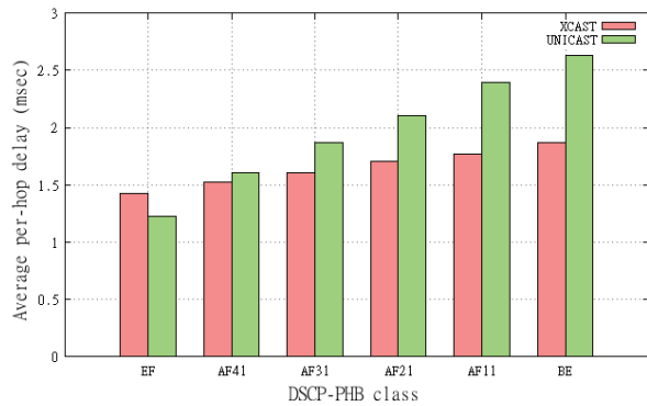
Figure 3. Comparative average per-hop delay
