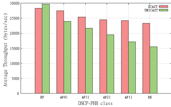
Figure 2. Comparative average throughput
