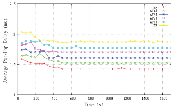
Figure 4. Average per-hop delay for XCAST
