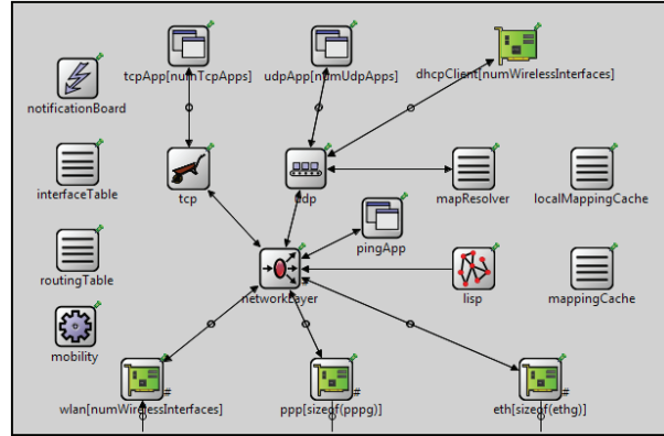
Figure 4: LISP mobile node in OMNeT++/INET.
