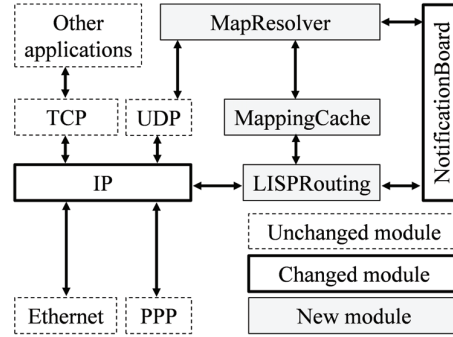
Figure 3: Architecture of a LISP gateway.
