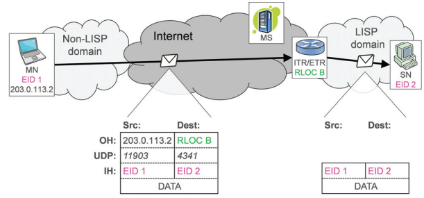
Figure 2: Packet flow sequence with LISP-MN.
