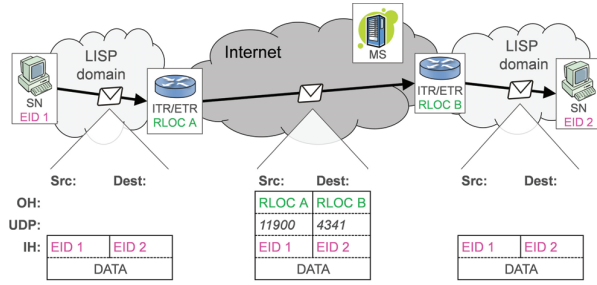
Figure 1: Packet flow sequence with LISP.
