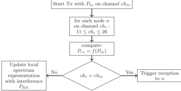
Figure 3: Interference in our multi-channel extension. Let f be a function describing the combined effect of path loss, shadowing and fading.
