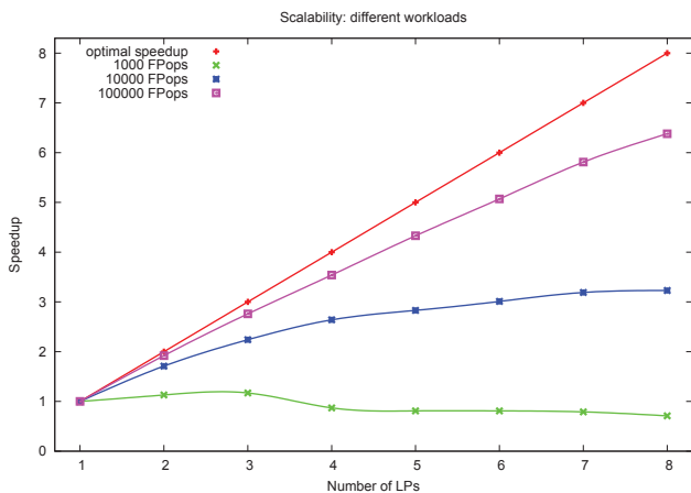
Figure 2: Speedup, increasing workload per entity, different configurations
