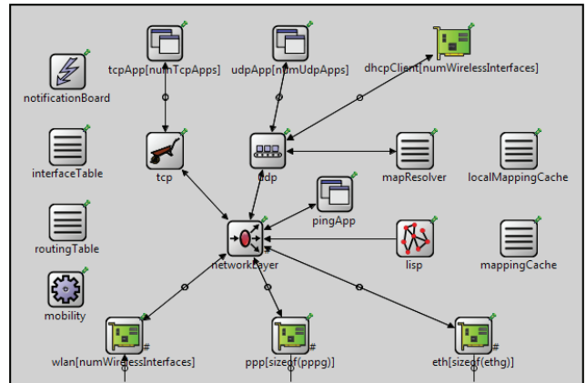
Figure 4: LISP mobile node in OMNeT++/INET.
