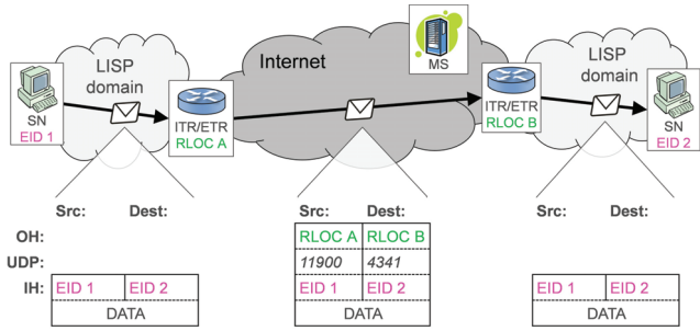
Figure 1: Packet flow sequence with LISP.
