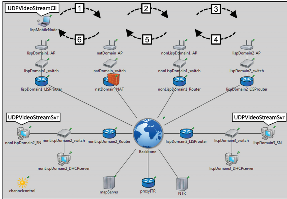
Figure 5: LISP mobile node moving from left-hand side to right-hand side and back. During its movement, the following handover events occur: (1) : LISP → NAT, (2) : NAT → nLISP, (3) : nLISP → LISP, (4) : LISP → nLISP, (5) : nLISP → NAT, (6) : NAT → LISP.
