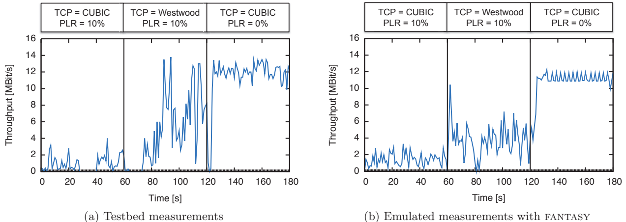
Figure 5: Comparison of throughput measurements for a cross-layer optimization scenario. TCP’s congestion control algorithm is changed based on the changing packet loss ratio (PLR) and the received signal strength indicator (RSSI).
