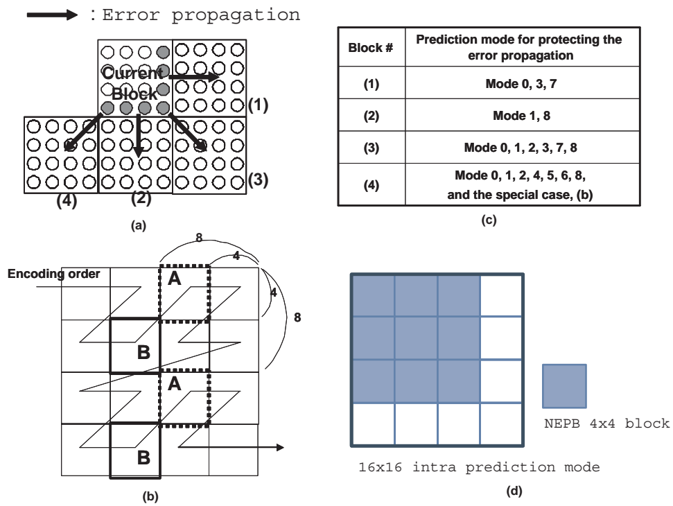
Figure 2: (a) Neighboring 4 \times 4 prediction blocks from the current one, (b) special case for Block-(4), (c) intra prediction modes for NEPB, (d) NEPB for 16 \times 16 intra prediction mode.
