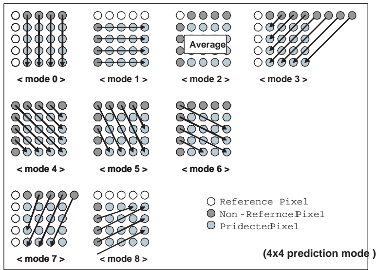
Figure 1: Intra prediction modes and referred boundary pixels for neighboring blocks.
