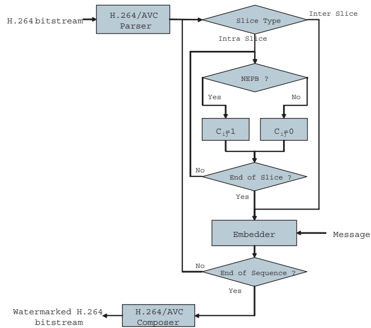
Figure 3: Flowchart for the proposed data embedding method.
