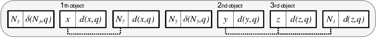
Figure 1: Snapshot of the priority queue at a given time during the execution of the DINN algorithm
