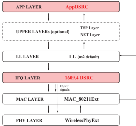
Figure 2: The revised Ns2.34 architecture.
