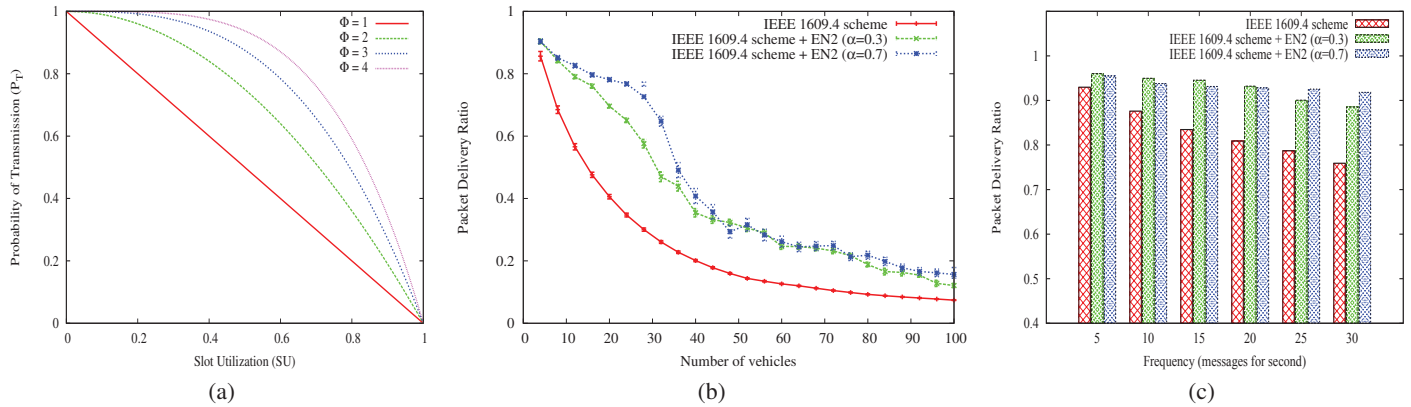
Figure 7: The P_T values as a function of the SU level are shown in Figure 7(a). The improvement produced by the EN2 scheme in terms of delivery ratio is shown in Figures 7(b) and Figure 7(c).
