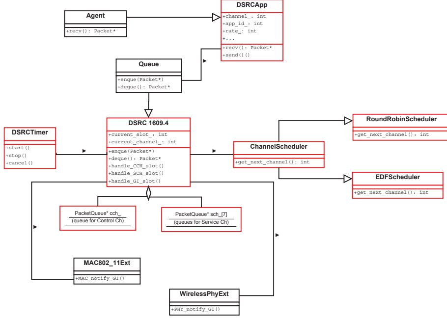
Figure 3: The class diagram of the IEEE 1609.4 implementation in ns2.
