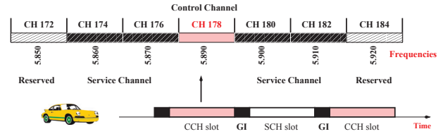
Figure 1: The DSRC spectrum frequencies and the IEEE 1609.4 WAVE protocol operations.
