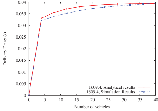
Figure 4: Analytical vs Simulation delivery delay.
