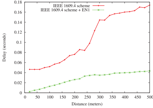
Figure 6: The improvement produced by the EN1 scheme in terms of delivery delay.
