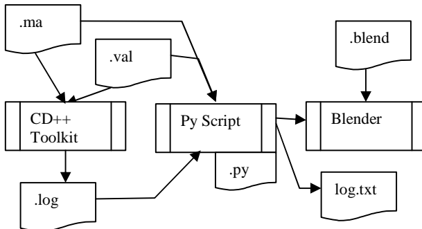
Figure 3: Visualization Architecture
