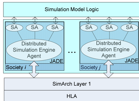
Figure 4 DisSimJADE architecture
