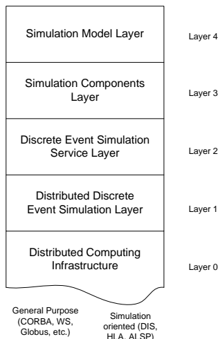
Figure 1 SimArch's layered architecture [4]
