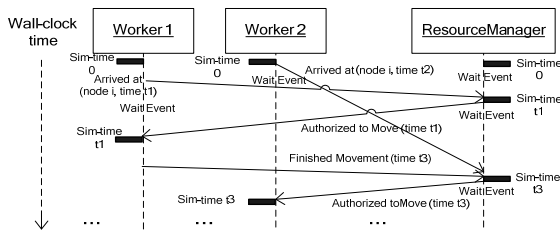
Figure 7 Example sequence diagram [24]
