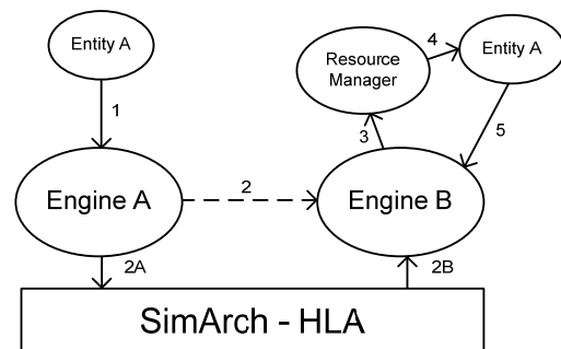
Figure 6 Example of agent mobility
