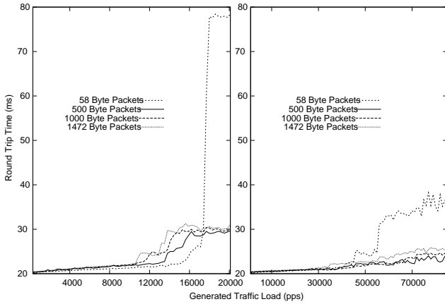
Figure 4: RTT overhead for Experiment 1.
