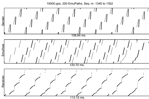
Figure 8: Snapshot of a run in Experiment 2.
