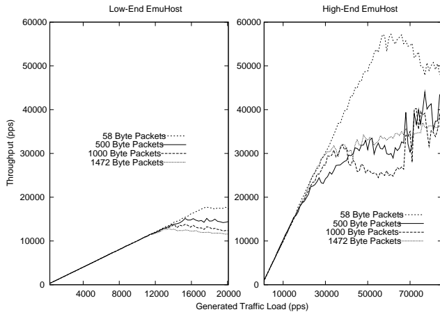
Figure 3: Throughput for Experiment 1.
