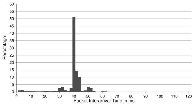
Figure 5: Packet Interarrival Time Distribution (overall)
