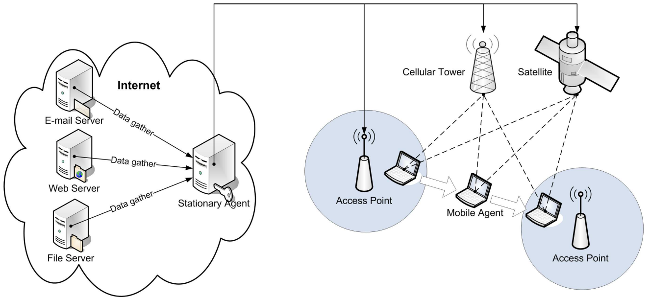
Figure 1: The architecture of a ParaNets-Enabled DBS-IC system.
