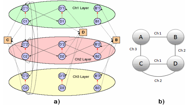
Figure 9a. Layered Graph model representing a sample 4 node network. 9b. Planar Graph model representing a sample 4 node network.
