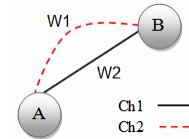
Figure 1. Nodes A and B linked by 2 edges.
