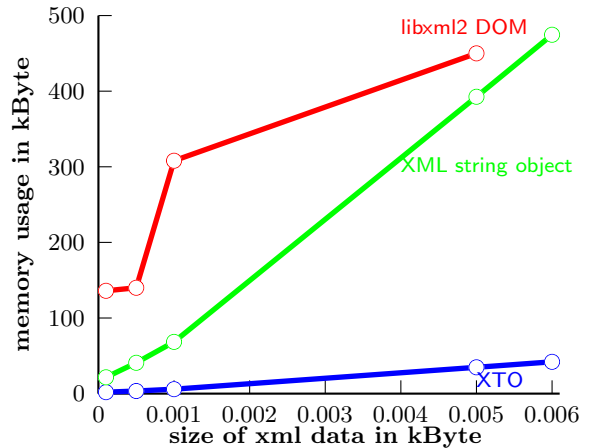
Figure 7: XMark XML Memory Usage
