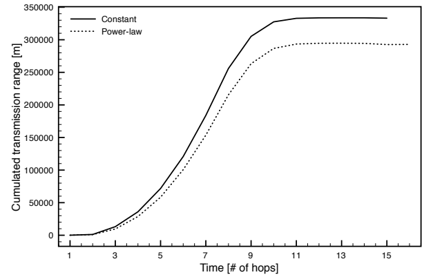
Figure 8: Cumulated transmission range, gossip ratio = 0.6
