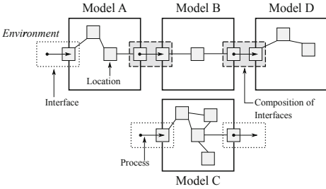
Fig. 1. Interfaces, composition, and substitution
