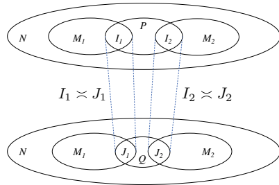
Fig. 2. Interfaces and substitution
