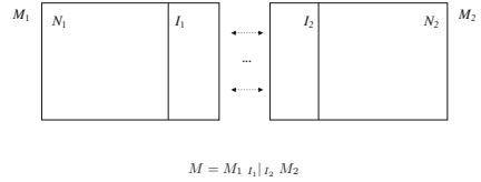
Fig. 6. Interfaces and local reasoning
