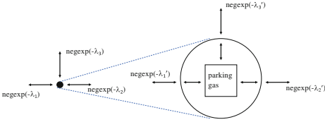
Fig. 5. Substitution
