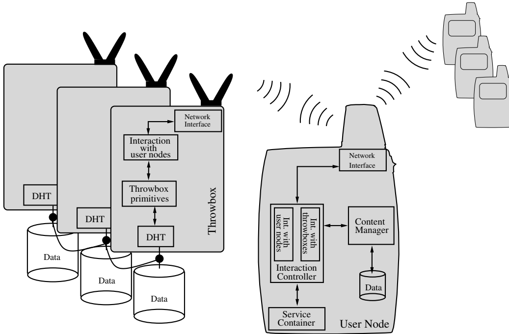
Figure 4: Functional blocks representation for the network components: throwboxes and user nodes.
