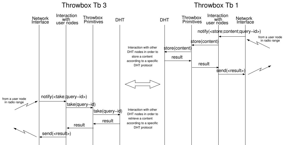
Figure 6: Interaction diagram for the sequence of operations involving throwboxes.
