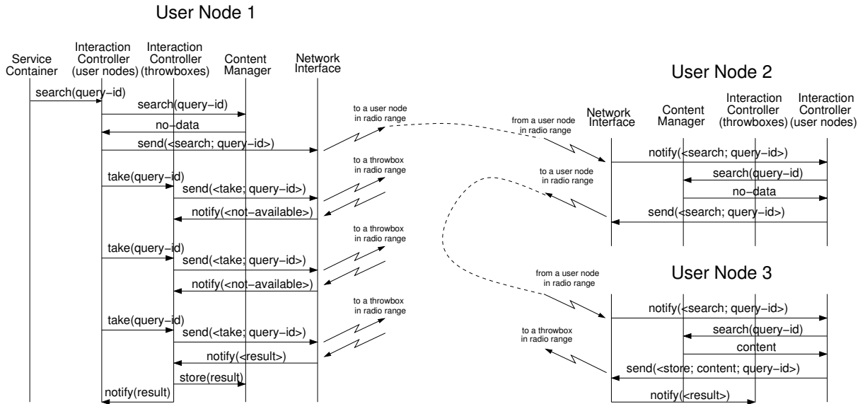
Figure 5: Interaction diagram for the sequence of operations involving user nodes.
