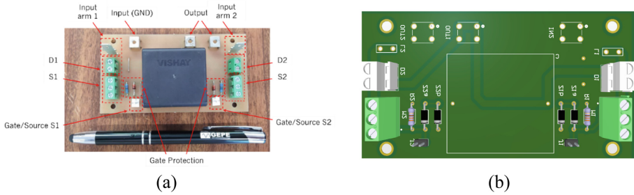
Fig. 8. PCB developed for the DC-DC converter of the interleaved boost type: (a) PCB; (b) Altium 3D model.
