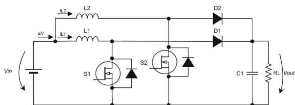
Fig. 3. Electrical schematic of the DC-DC IBC with two arms.
