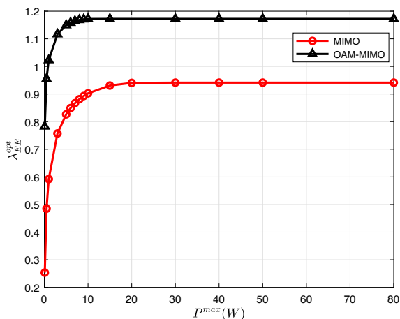
Fig. 3. The EE trend of the OAM-MIMO system and the MIMO system with the variation of P^{max} .
