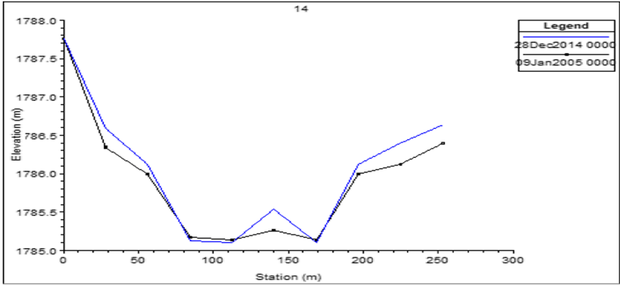
Fig. 11. Bed change plot for 10-year simulation period according to Wilcock-Crowe
