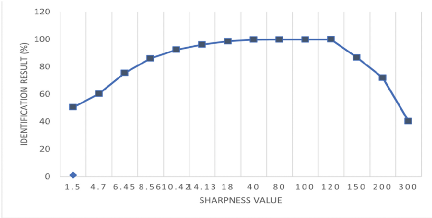
Fig. 8. Accuracy vs. sharpness value.
