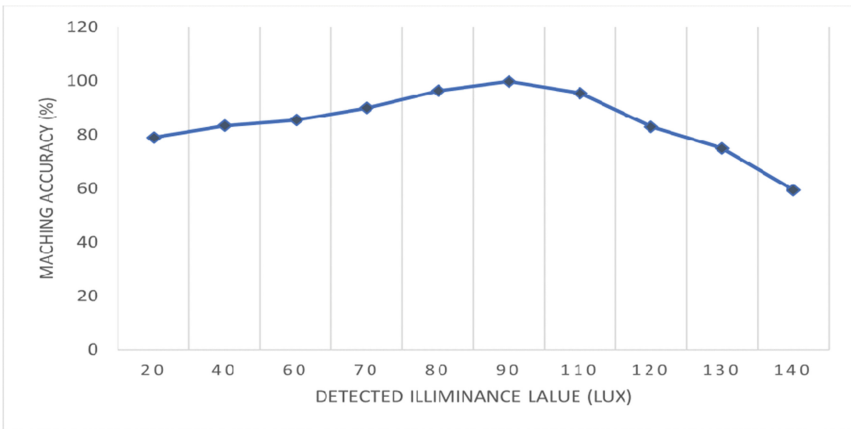
Fig. 9. Accuracy vs. detected image illuminance.
