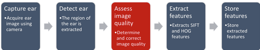
Fig. 2. Proposed ear recognition approach.
