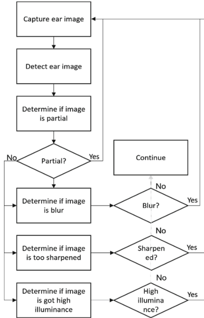
Fig. 3. The proposed ear recognition flow.
