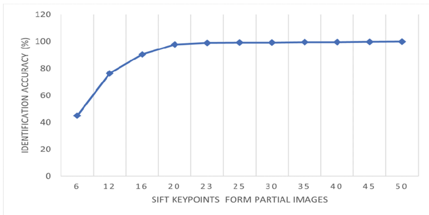
Fig. 7. Accuracy vs. number of sifting key points.
