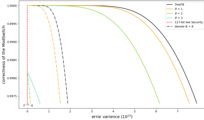
Fig. 4. Error rate of Tree-BML and TreeFB algorithm
