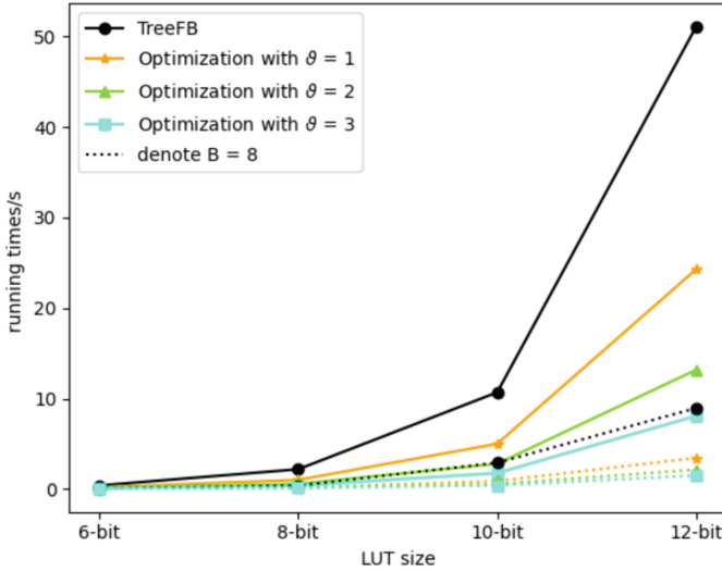
Fig. 2. Calculation of LUT
