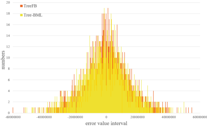
Fig. 3. Interval statistics of values of output error
