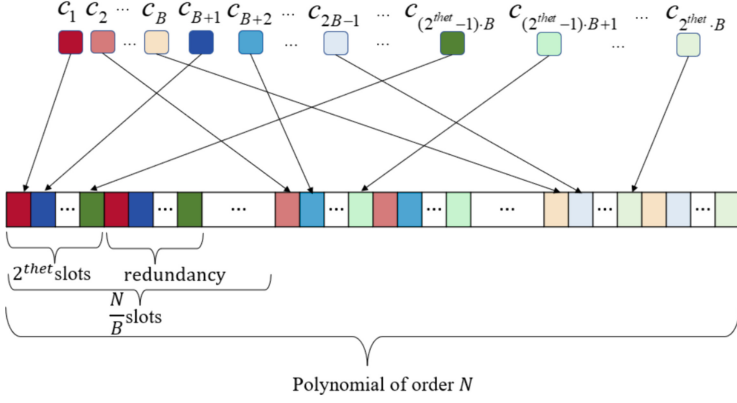
Fig. 1. Compression of 2^{\theta} B TLWE ciphertexts
