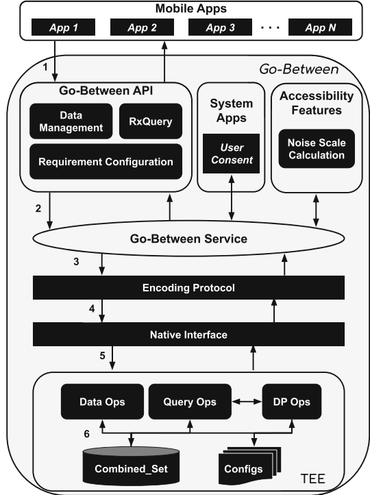
Fig. 2. System architecture.
