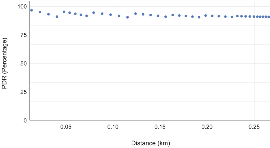
Fig. 11. High load (density \rho of 900 nodes per \text{km}^2 , traffic intensity of 1/2 \text{ min}^{-1} ), SF boundaries for target PDR of 90%, Rayleigh fading. Cell capacity around 200 nodes.
