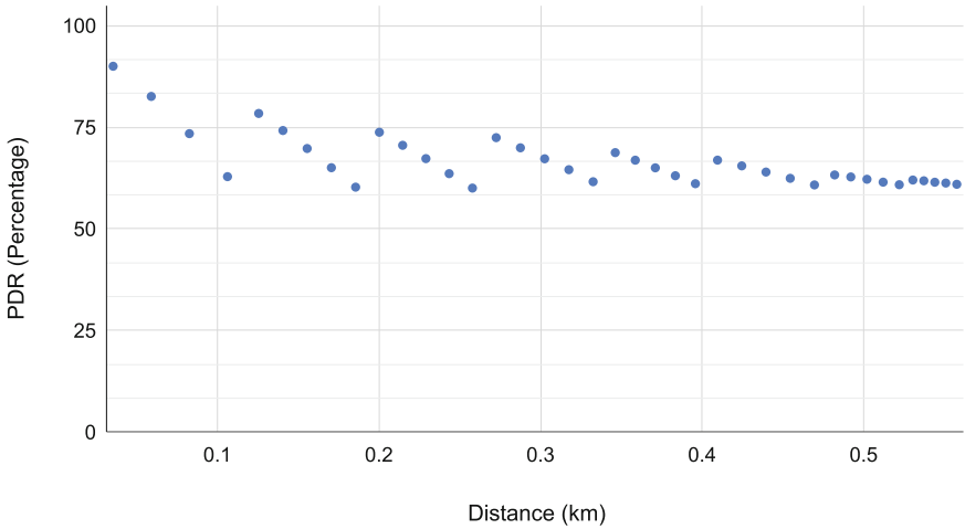
Fig. 10. High load (density \rho of 900 nodes per \text{km}^2 , traffic intensity of 1/2 \text{ min}^{-1} ), SF boundaries for target PDR of 60%, Rayleigh fading. Cell capacity around 880 nodes.
