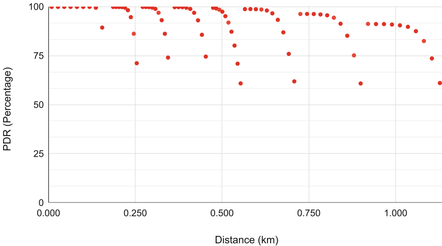
Fig. 4. Low load (density \rho of 90 nodes per km 2 , traffic intensity of 1/12.33 min -1 ), SF boundaries for target PDR of 60%, Rician fading. Cell capacity around 360 nodes.
