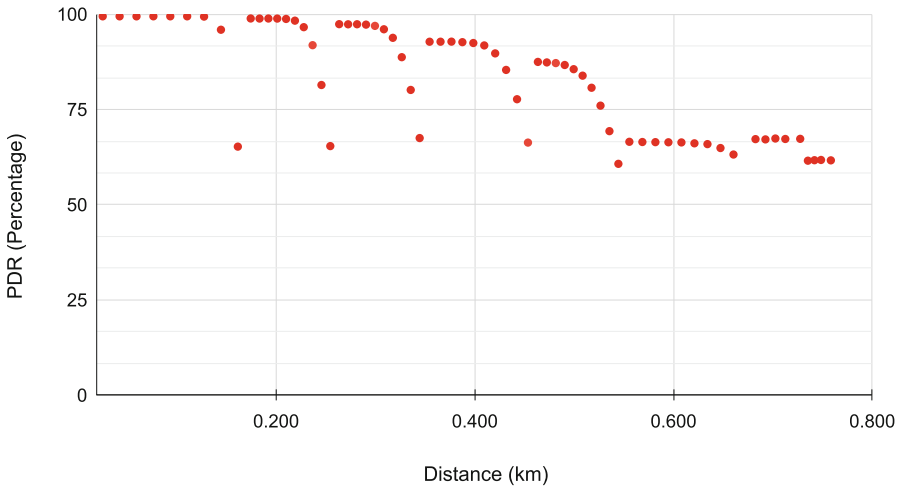
Fig. 6. High load (density \rho of 900 nodes per \text{km}^2 , traffic intensity of 1/2 \text{ min}^{-1} ), SF boundaries for target PDR of 60%, Rician fading. Cell capacity around 1620 nodes.
