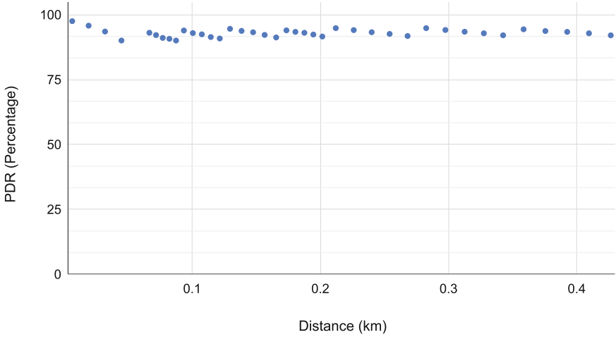
Fig. 9. Low load (density \rho of 90 nodes per \text{km}^2 , traffic intensity of 1/12.33 \text{ min}^{-1} ), SF boundaries for target PDR of 90%, Rayleigh fading. Cell capacity around 50 nodes.
