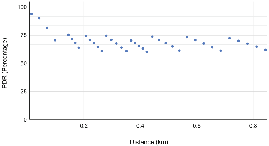
Fig. 8. Low load (density \rho of 90 nodes per \text{km}^2 , traffic intensity of 1/12.33 \text{ min}^{-1} ), SF boundaries for target PDR of 60%, Rayleigh fading. Cell capacity around 200 nodes.
